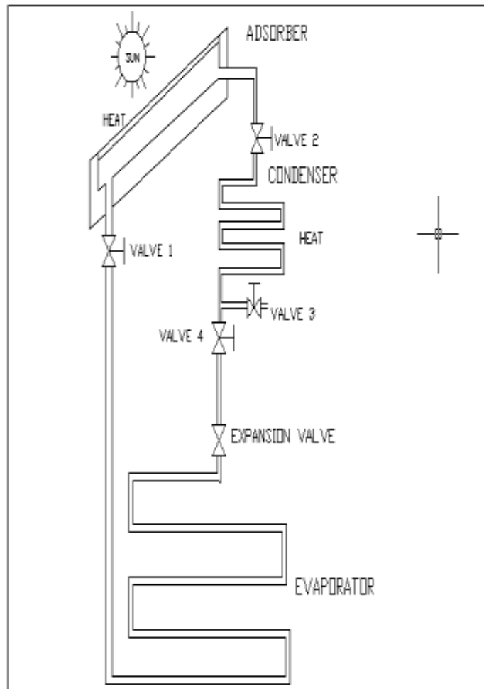
Fig -2: Diagram of set up with valve arrangement
